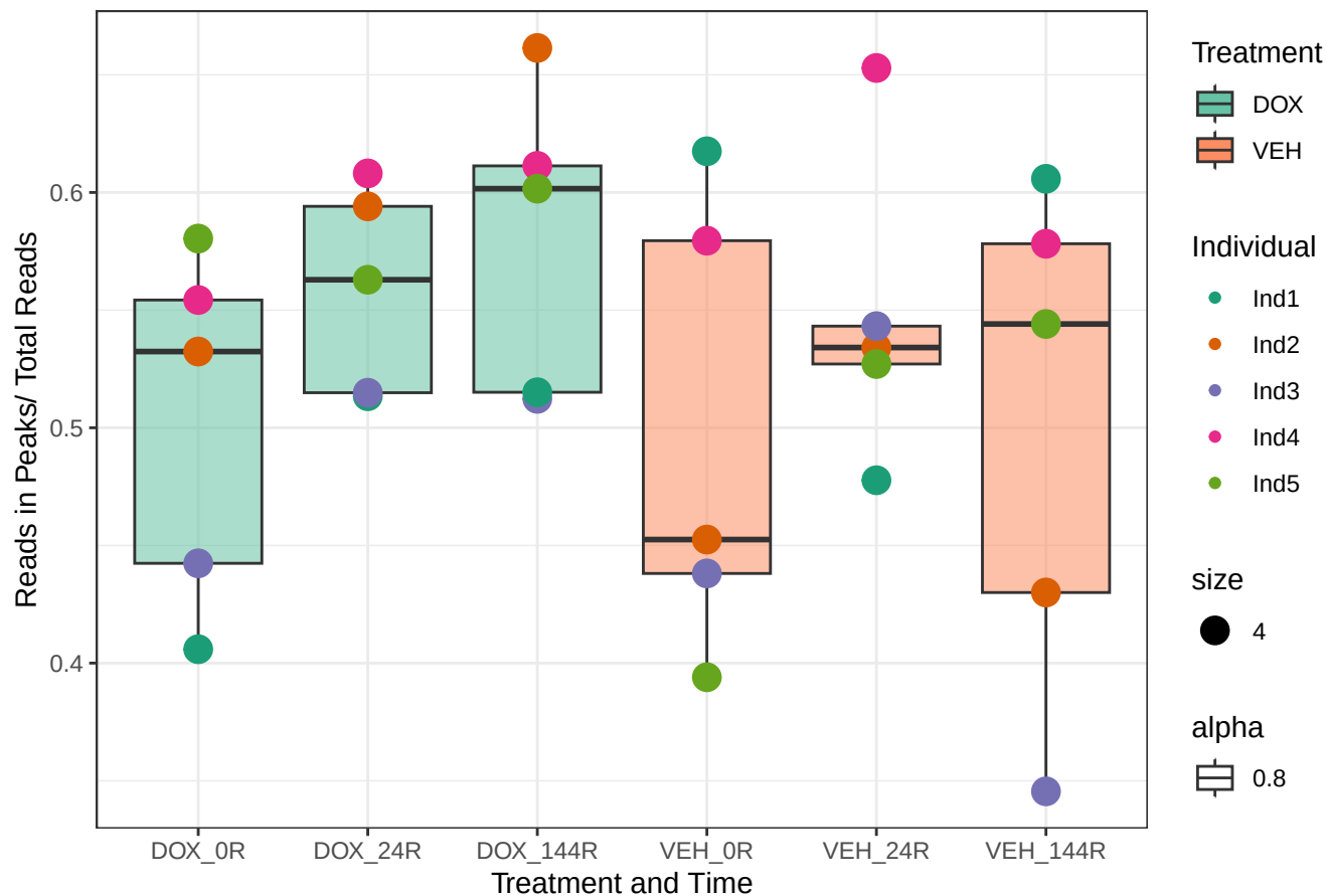
Fraction of Reads in Peaks for H3K27ac
